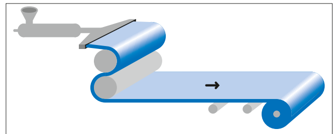
Schematic diagram of flat film extrusion.
