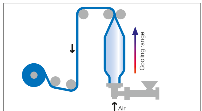
Schematic diagram of blown film extrusion.
